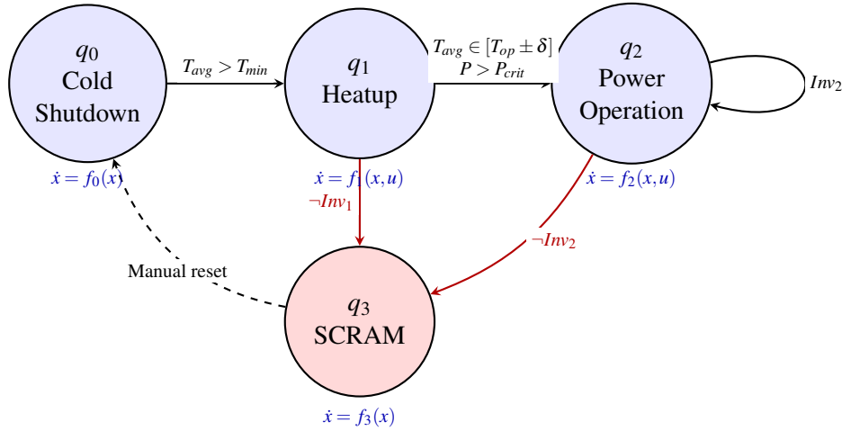
Figure 1: Simplified hybrid automaton for reactor startup. Each discrete state q_i has associated continuous dynamics f_i . Guard conditions on transitions (e.g., T_{avg} > T_{min} ) are predicates over continuous state. Invariant violations ( \neg Inv_i ) trigger transitions to the SCRAM state. The operational level manages discrete transitions; the tactical level executes continuous control within each mode.
