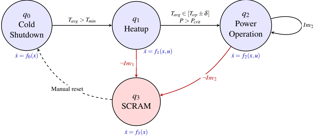
Figure 1: Simplified hybrid automaton for reactor startup. Each discrete state q_i has associated continuous dynamics f_i . Guard conditions on transitions (e.g., T_{avg} > T_{min} ) are predicates over continuous state. Invariant violations ( \neg Inv_i ) trigger transitions to the SCRAM state. The operational level manages discrete transitions; the tactical level executes continuous control within each mode.
